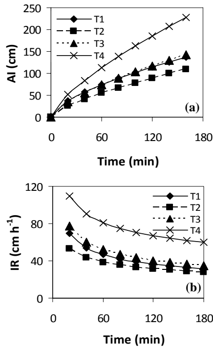
Figure 5. Curves of (a) accumulated infiltration (AI) and (b) infiltration rate (IR).
