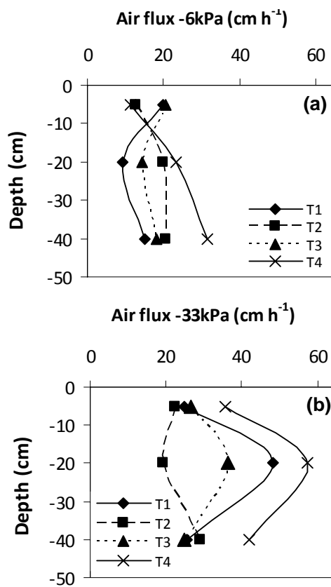
Figure 4. Air flux for each treatment, in samples equilibrated at a water suction of (a) -6 and (b) -33 kPa.
