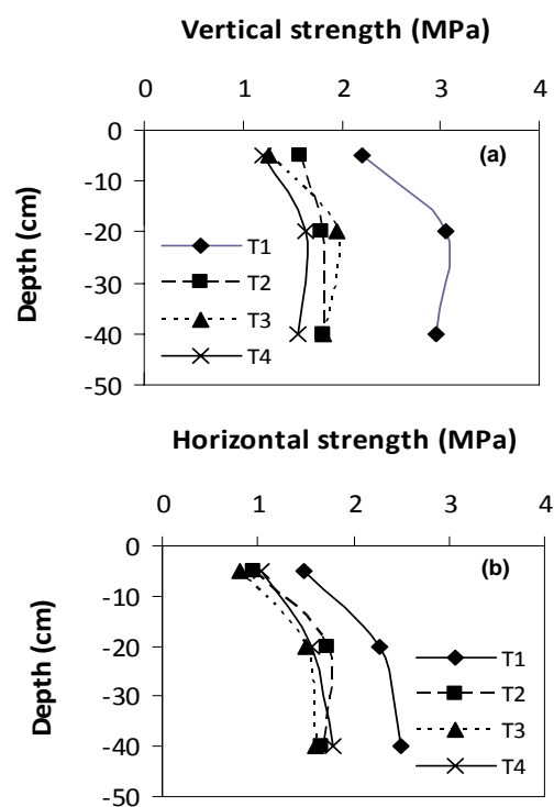
Figure 3. Penetration resistance (MPa) as a function of depth. Vertical (a) and horizontal (b) values measured one day after irrigation.
